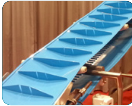
Special cleats on trough conveyor
