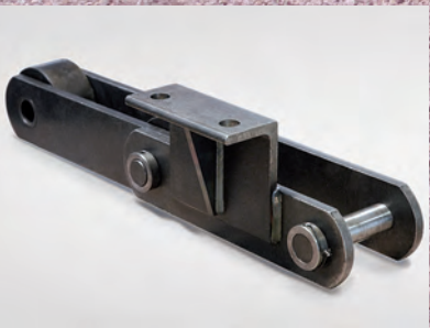
Twin Stranded Bushed Chain with Plain Roller and Welded Attachment Bracket
