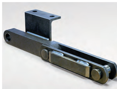
Twin Strand Block Chain with Attachment Bracket and Wear Strip welded to the Block Link
