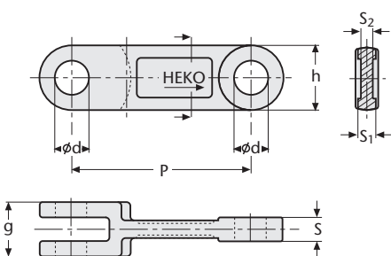
Single Strand Forged Link Chain with Welded Scraper
